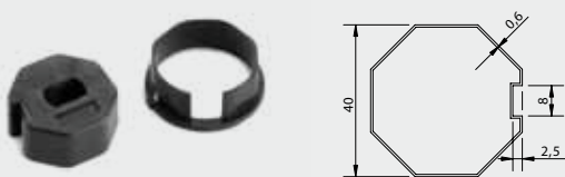
MS35 AP 01N 0B 00 Puleggia/corona per tubo ottagonale Ø40 Male/female adapter for Ø40 mm octagonal tube
