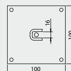
MS59 AS 04N 0G 00 Staffa di supporto quadra - Zincato Bianco Square section support bracket - White Galvanized
