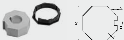
MS59 AP 01N 0B 00 Puleggia/corona per tubo ottagonale Ø70 Male/female adapter for Ø70 mm octagonal tube
