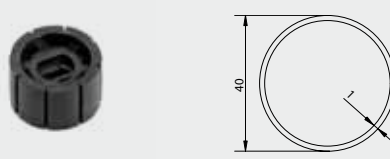
MS35 AP 02N 0B 00 Puleggia/corona per tubo tondo Ø40 Male/female adapter for Ø40 mm round tube
