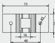
MS59 AS 03N 0G 00 Staffa di supporto max 100Nm interasse 48 mm - Zincato Bianco Support bracket, max 100Nm centre distance 48 mm - White Galvanized
