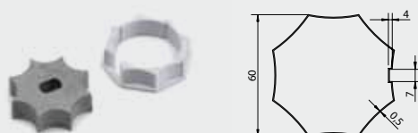
MS45 AP 04N 0B 00 Puleggia/corona per tubo a stella Ø60 Male/female adapter for Ø60 mm star-section tube
