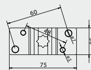
MS45 AS 02N 0G 00 Staffa di supporto max 30Nm interasse 48 mm - Zincato Bianco Support bracket, max 30Nm centre distance 48 mm - White Galvanized
